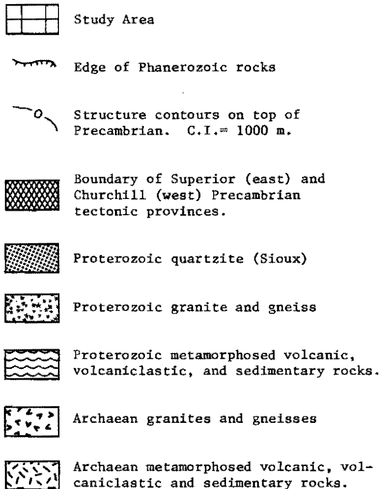
Fig. 1. Area covered by Red River Valley Drilling Project (Moore 1978), and general tectonic features redrawn from King (1969).
